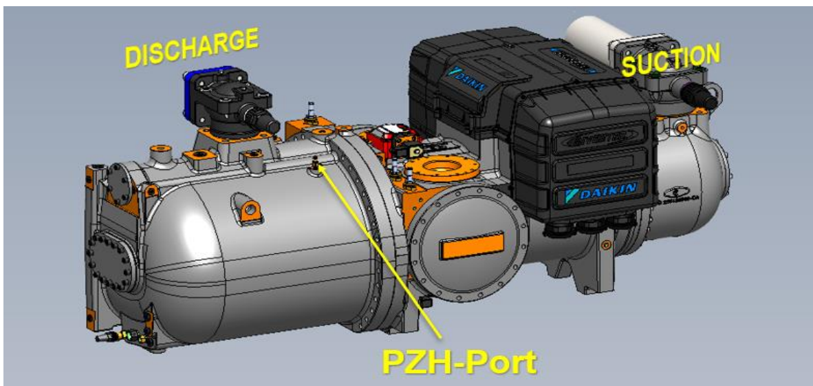
Figure 2 F4AL Compressor
