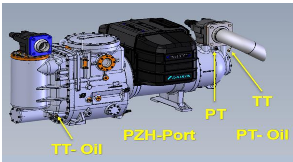
Figure 3 310240 Compressor
