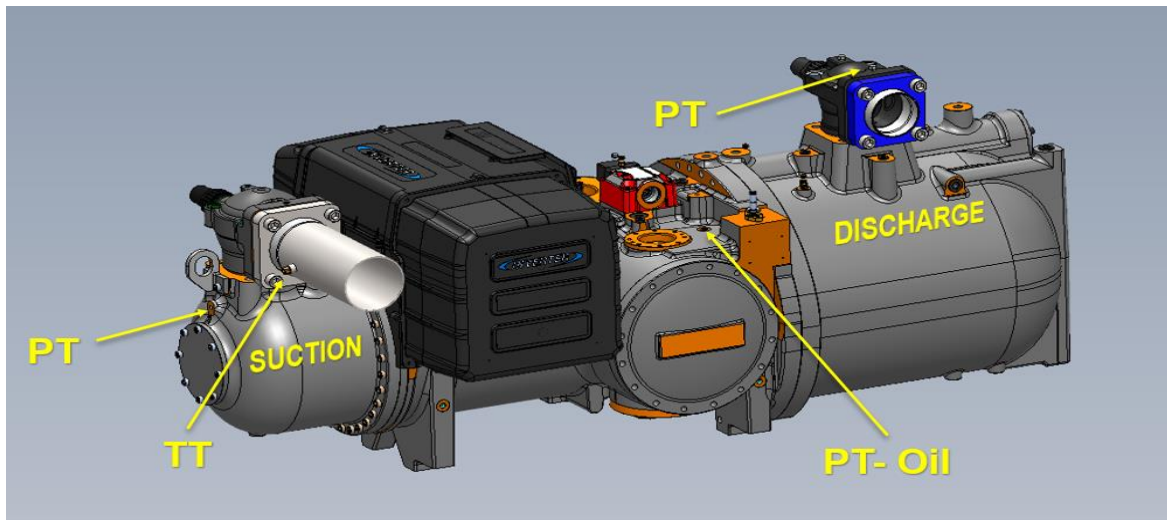
Figure 1 F4AL Compressor
