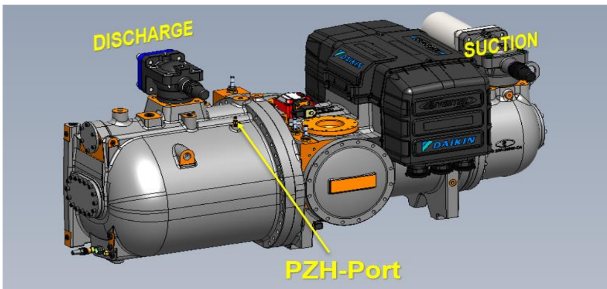
Figure 2 F4AL Compressor
