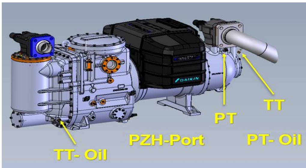
Figure 3 310240 Compressor
